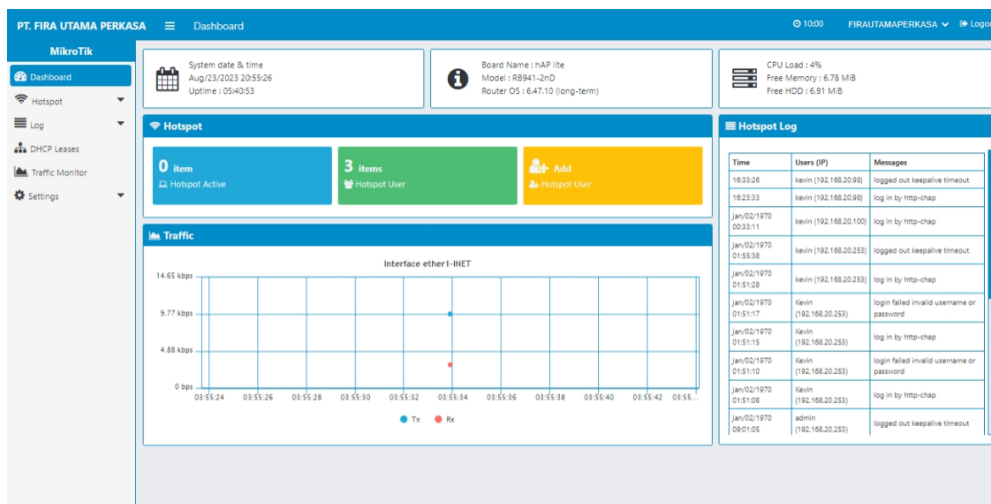
Fig 4: Tampilan Monitoring
